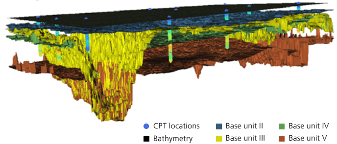
Geological model
